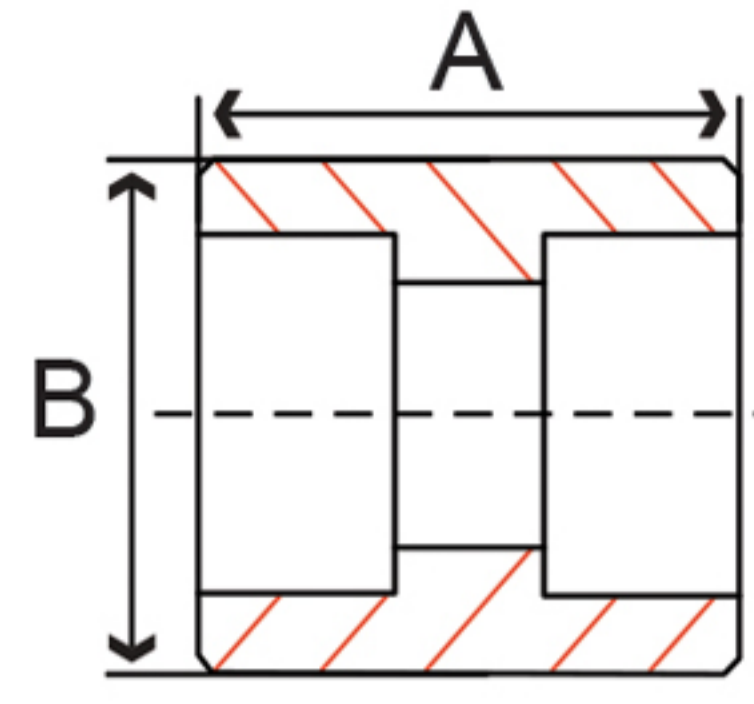
Fig. 52CP3 – Coupling
